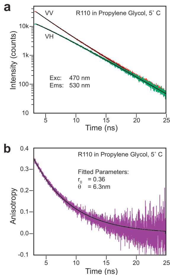
Fig. 4. Fluorescence anisotropy decay. Time-domain measurements of a fluorescence anisotropy decay of rhodamine 110 in propylene glycol. (a) Fluorescence intensity decays of polarized components, (b) calculated anisotropy decay.
