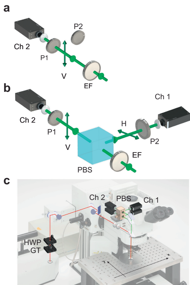
Fig. 5. Detection schemes. Detection schemes for fluorescence anisotropy measurements. In the L-format (a) all fluorescence intensities are measured using a single channel, sequentially, by replacing the analyzer P1, with the orthogonal one P2. In the T format (b) fluorescence intensities are measured simultaneously on two different channels (Ch1 and Ch2), by two different PMTs. The format is therefore more suited for rapid in vitro and in vivo imaging. (c) Scheme of principle of a two photon fluorescence anisotropy microscopy imaging system. GT, Glan-Thompson polarizer; HWP half-wave plate; PBS polarization beam splitter, EF emission filter.
