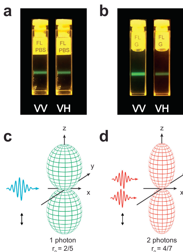
Fig. 2. One-photon and Two-photon fluorescence anisotropy. Images of fluorescence anisotropy for fluorescein. (a) In PBS, the rotational diffusion of the excited molecules is occurring on a time scale shorter than the fluorescence lifetime, and tends to scramble the orientation of the emission dipoles. No preferential emission direction is present. (b) In glycerol, the molecular rotation is occurring on a time scale slower than the fluorescence lifetime. A strong degree of fluorescence emission anisotropy is present. (c, d) Photoselection function for one- (a) and two-photon (b) excitation. The one-photon fundamental anisotropy is equal to 2/5 . The two-photon fundamental anisotropy is higher and equal to 4/7 , due to two-photon photoselection. Adapted with permission from [255], Nature Publishing Group.
