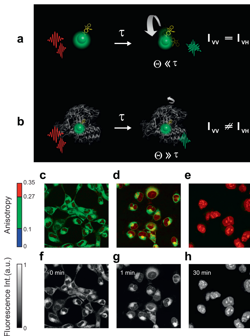
Fig. 6. Two-photon fluorescence anisotropy imaging of drug-target engagement. (a,b) Comparison between the rotation of the free fluorescently labeled drug (PARPi-FL) in solution and when bound to its target (PARP). Due to the large difference in molecular weight between the target (ca. 120 kDa) and the small molecule, the fluorescence anisotropy of the drug-target complex will increase following two-photon excitation ( \Theta \gg \tau ). (c,h) Temporal evolution of the fluorescence anisotropy (c–e) and intensity (f–h), for HT1080 cells incubated with PARPi-FL, at three representative time points during loading and washing phases. Adapted with permission from [255], Nature Publishing Group.
