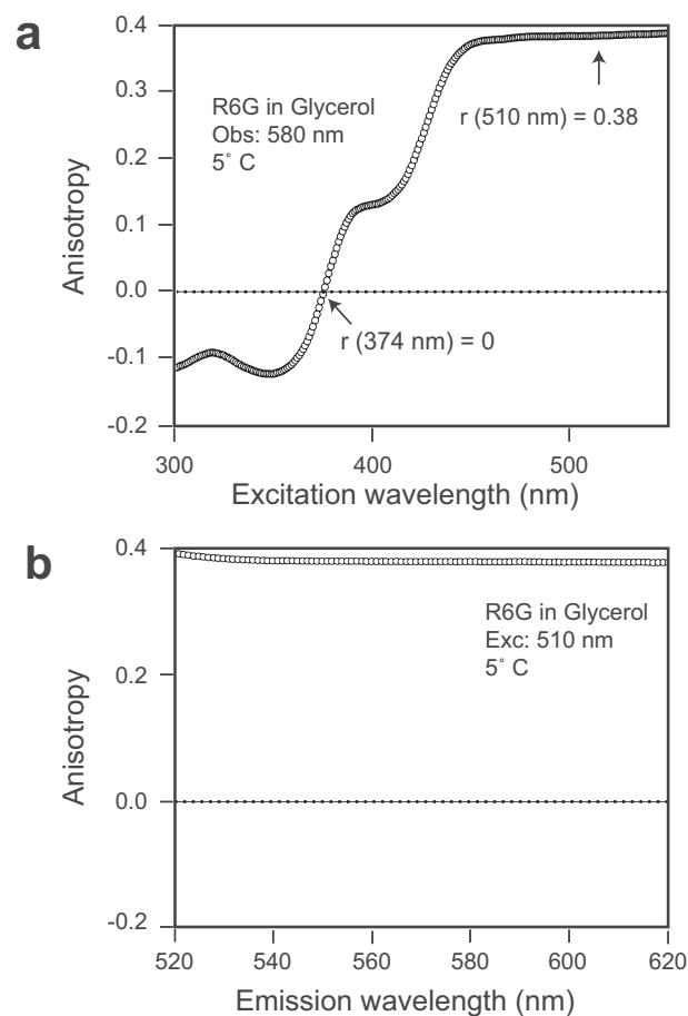
Fig. 3. Fluorescence anisotropy spectra. Fluorescence anisotropy spectra of rhodamine 6G. (a) in excitation wavelengths, (b) in emission wavelengths. Note that below 374 nm the fluorescence anisotropy of rhodamine 6G is negative which indicates excitation to higher electronic state with perpendicular orientation of absorption transition moment.
