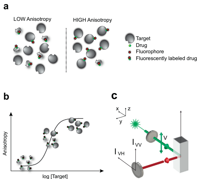
Fig. 1. Fluorescence anisotropy fundamentals. (a) Upon binding to its target, the fluorescently labeled small molecule drug presents an increase in anisotropy. (b) Titration and measurements of fluorescence anisotropy, enable accurate reconstruction of binding isotherms. (c) Standard optical arrangement for measurements of fluorescence anisotropy. The subscript letters V and H, stand for vertical and horizontal. The first subscript, indicates the direction of polarization of the excitation light. The second subscript, indicates the direction of polarization of the emission polarizer. Adapted with permission from [255], Nature Publishing Group.
