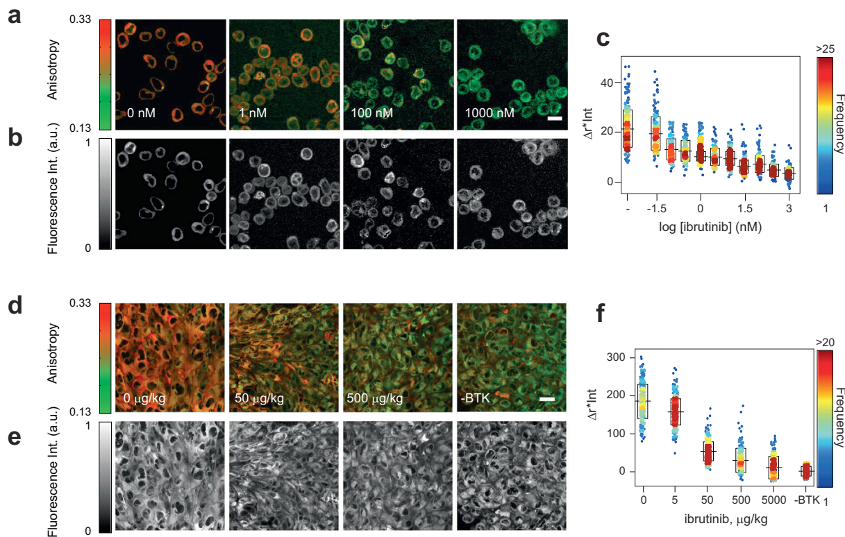
Fig. 9. Competitive binding of matched fluorescently labeled drugs. Fluorescence anisotropy (a) and intensity (b) images of Toledo cells in vitro , loaded at different concentration of ibrutinib, followed by ibrutinib-BFL. (c) Measurements on single cells cytoplasm after segmentation, of \Delta r^*Int , at varying concentration of ibrutinib, followed by ibrutinib-BFL. Fluorescence anisotropy (d) and intensity (e) of HT1080 BTK-mCherry and BTK free HT1080 H2B apple dorsal window chamber tumors, following systemic ibrutinib delivery, and ex vivo ibrutinib-BFL loading. (f) Measurements on single cells cytoplasm after segmentation, of \Delta r^*Int , at varying concentration of ibrutinib delivery, following ibrutinib-BFL loading. Adapted with permission from [33], Nature Publishing Group.
